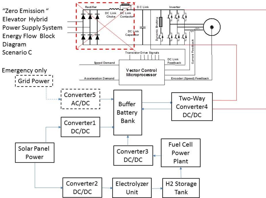
Figure 7 Energy Flow Block Diagram – Scenario C
