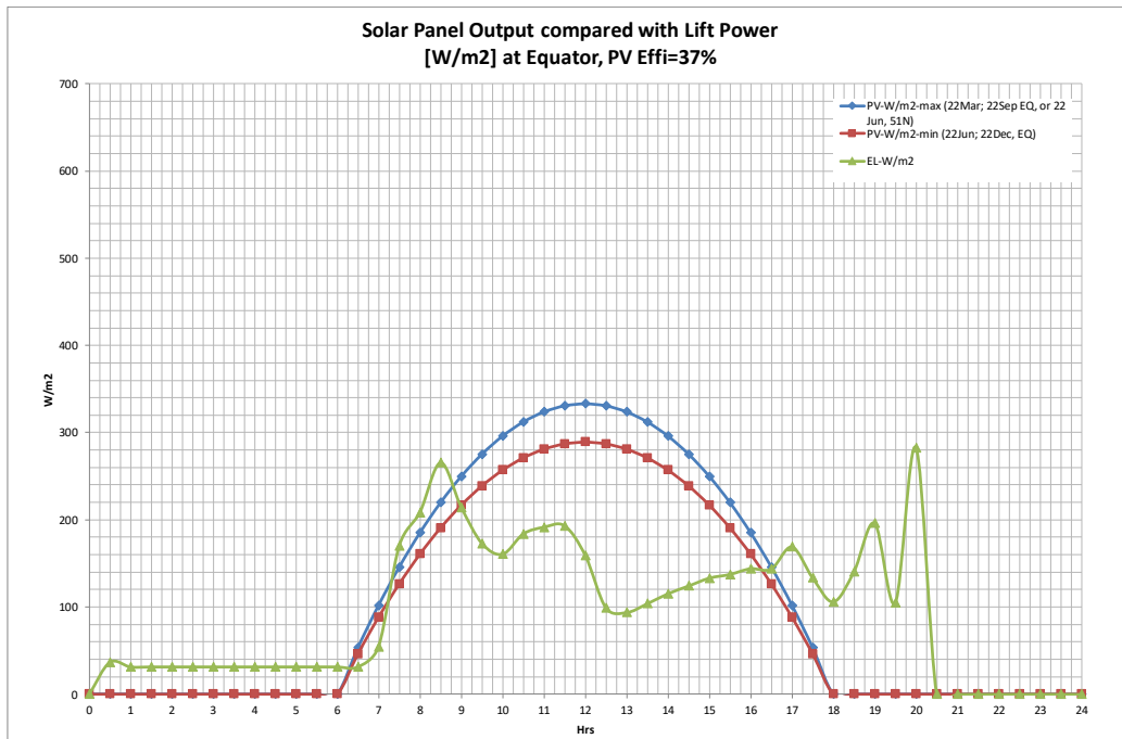
Figure 8 Lift daily energy requirement balanced with PV daily energy on 22 Jun at equator
