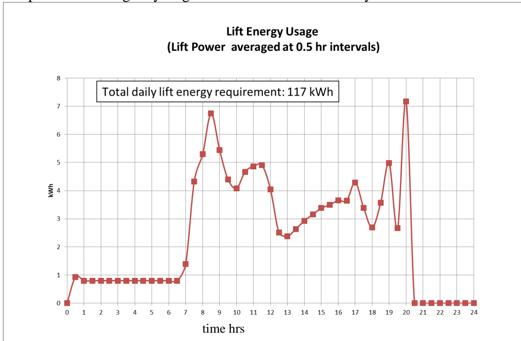
Figure 5 Lift energy consumption
