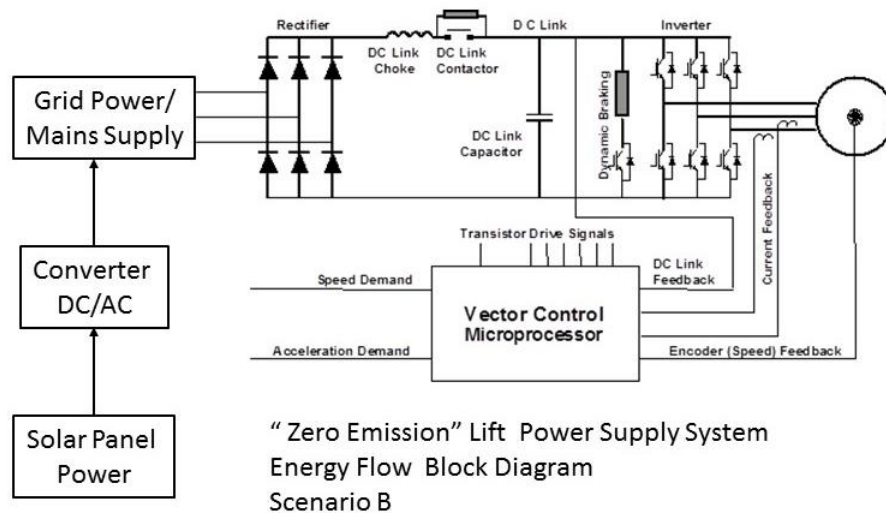
Figure 6 Energy Flow Block Diagram – Scenario B
