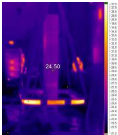
Figure 8 Thermographic picture. MRL control panel.
