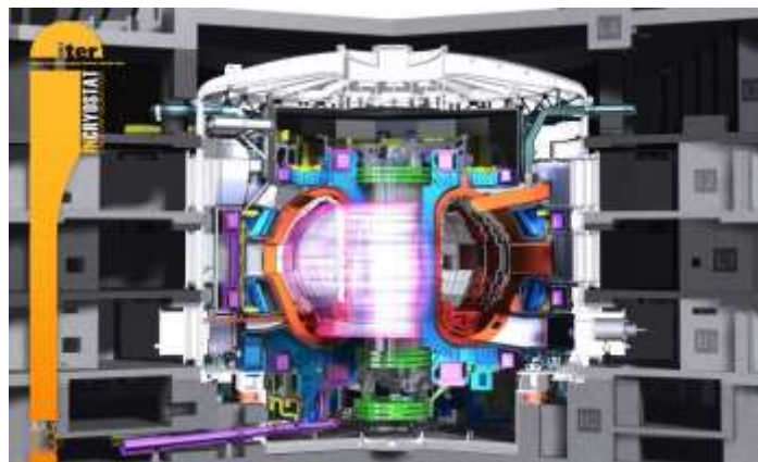
Figure 3 Tokamak machine diagram
